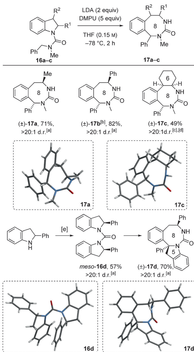
Scheme 5. Diastereoselective ring expansions. [a] d.r. was determined by ^1\text{H} NMR of the crude reaction mixture. [b] The relative chemistry of ( \pm )- 17b was assigned in analogy to ( \pm )- 17a . [c] d.r. of purified product. [d] Reaction run without DMPU. [e] Reaction conditions: Triphosgene (1.2 mmol) treated with pyridine (2.6 mmol) in anhydrous \text{CH}_2\text{Cl}_2 (0.7 M) at -78^{\circ}\text{C} . 2-Phenylindoline (2.6 mmol) added and reaction warmed to RT. 2-Phenylindolinecarbamoyl chloride (0.78 mmol) treated with 2-phenylindoline (1.0 mmol) and triethylamine (1.24 mmol) in anhydrous MeCN (0.4 M) at RT.
